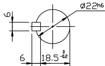
OUTPUT SHAFT
